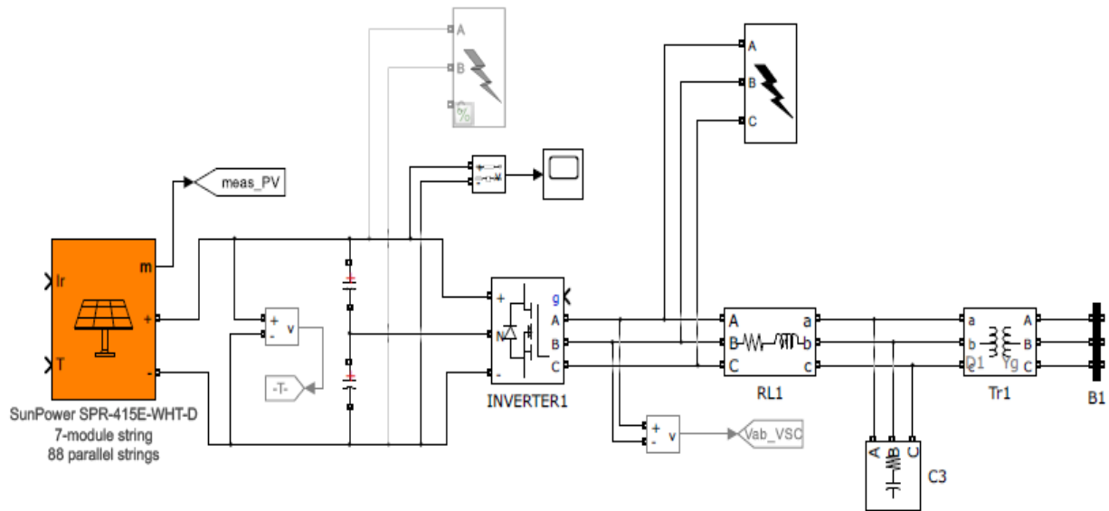
Fig 9. Simulation of a direct stroke on the DC side or the AC side of the inverter
