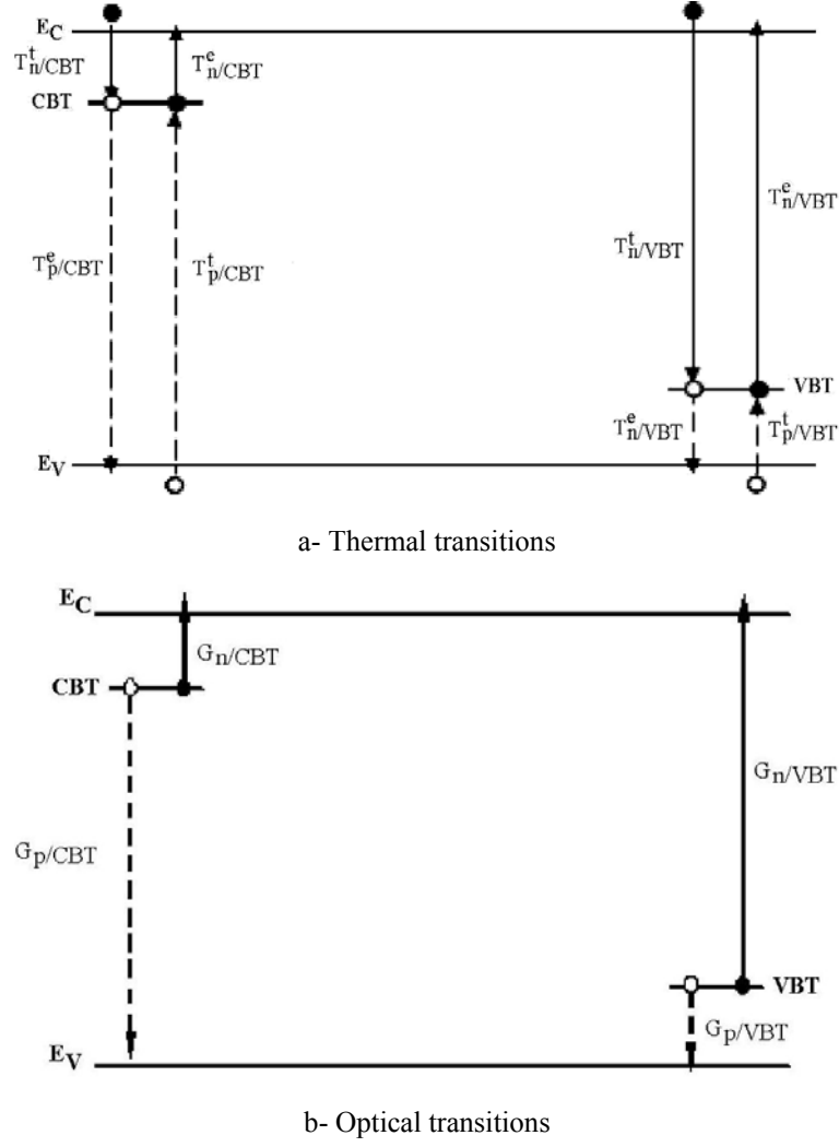
Fig. 1: Carrier transitions involved in the CPM simulation
