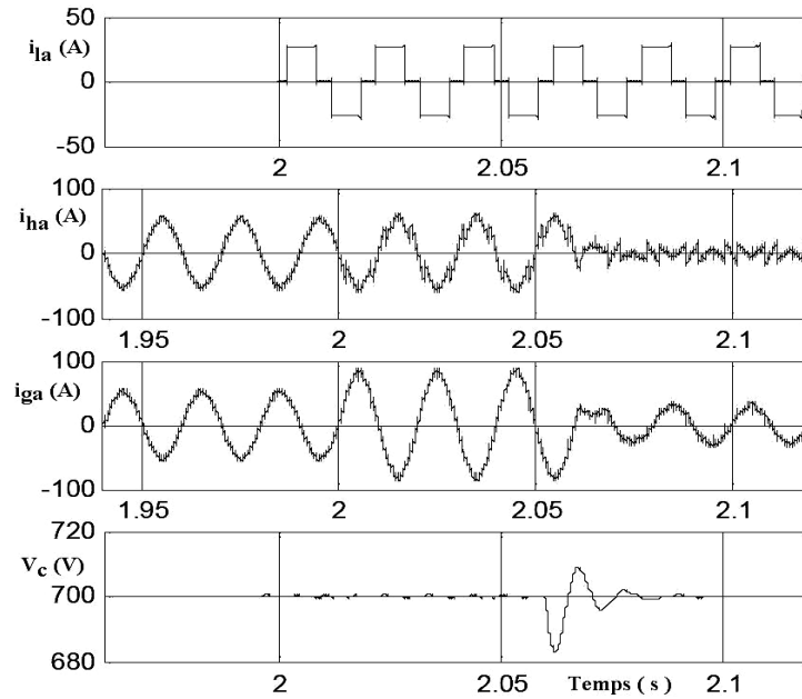
Fig. 4: Load current i_l , grid converter current i_{ha} , grid current i_{ga} , DC voltage V_c
