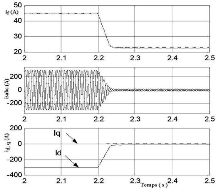
Fig. 8: Rotor current i_f , Stator currents i_{sabc} , Stator currents i_{dq} in dq co-ordinates with LC filter
