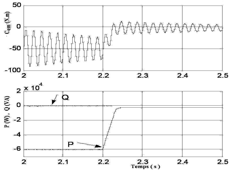
Fig. 9: Electromagnetic torque C_{em} , P and Q active and reactive power generated by SG with LC filter
