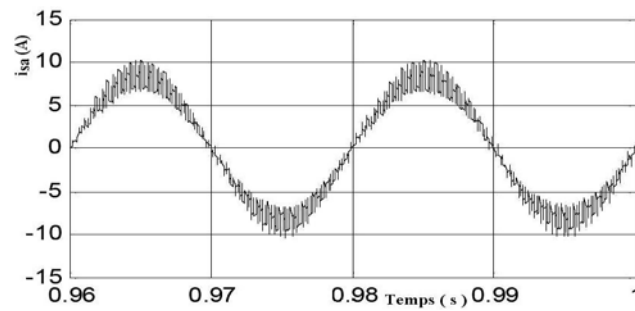
Fig. 10-a: SG's stator current performances without the LC filter
