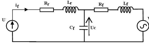
Fig. 3: Equivalent circuit of rotor-LC filter system
