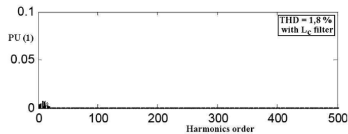
Fig. 10-d: SG's stator current harmonic spectrum with the LC Filter
