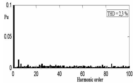
Fig 5b: Current harmonic spectrum after filtering
