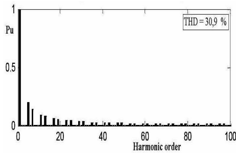
Fig. 5a: Load current harmonic spectrum before filtering
