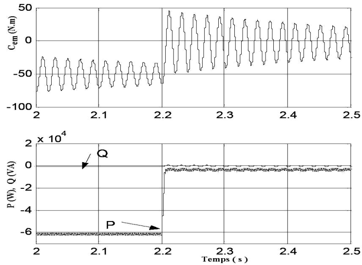
Fig. 7: Electromagnetic torque C_{em} , P and Q active and reactive power generated by SG without LC filter
