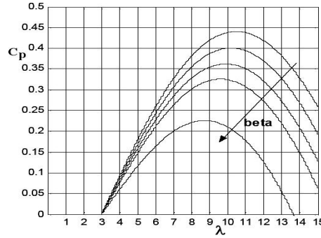
Fig. 1: C_p characteristics of wind turbine
