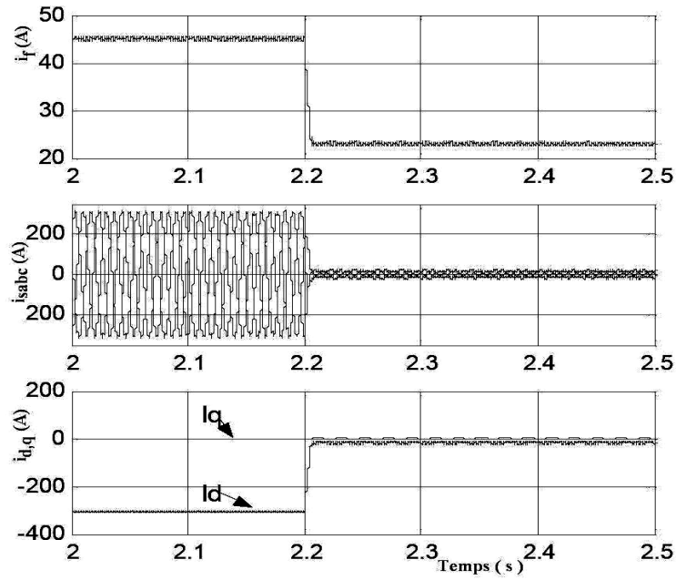
Fig. 6: Rotor current i_r , Stator currents i_{sabc} , stator currents i_{dq} in dq co-ordinates without LC filter
