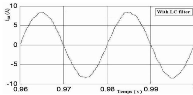
Fig. 10-c: SG's stator current performances with the LC filter
