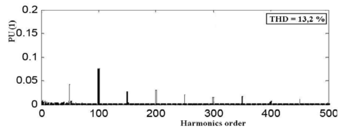
Fig. 10-b: SG's stator current harmonic spectrum without the LC Filter
