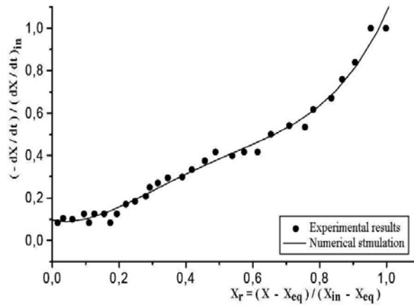
Fig. 1: Characteristic drying curves of apple slices
