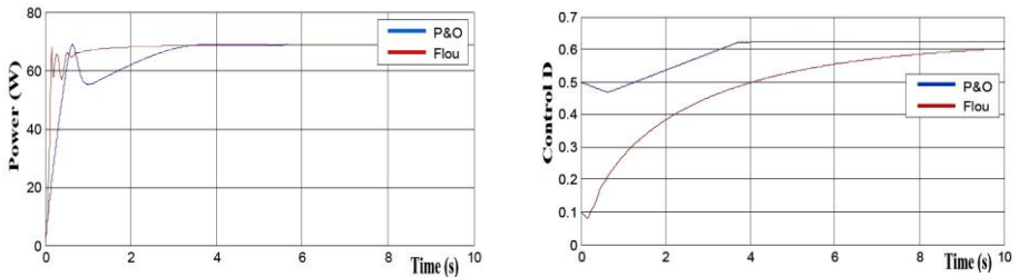
Fig. 8: Provided power from P&amp;O tracker and FLC Controller in a standard condition
