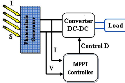
Fig. 3: Photovoltaic systems
