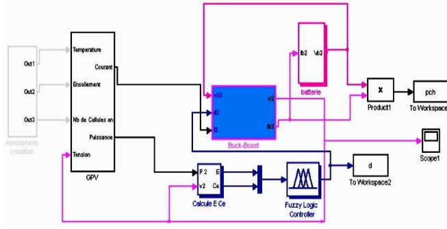
Fig. 6: Model SIMULINK of MPPT controller flow
