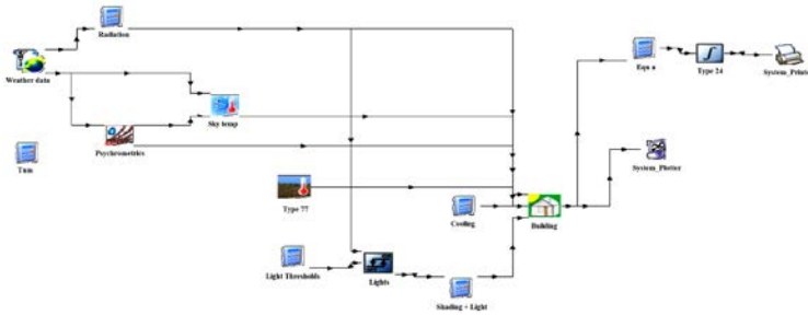
Fig. 1: Modules assembly for building description in TRNSYS
