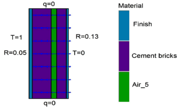
Fig. 6: Boundary conditions of double-walls without thermal bridge
