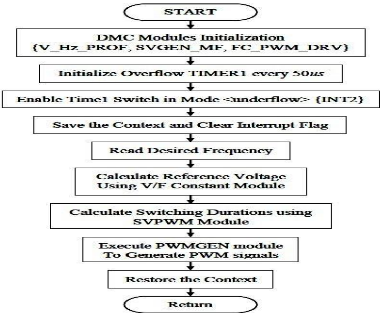
Fig. 9: Program Flowchart
