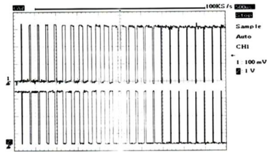
Fig. 10: PWM signal and its complement
