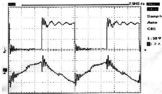
Fig. 13: Voltage and current waveforms for one IGBT cell
