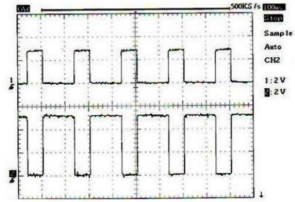
Fig. 12: PWM signals before and after optocouplers
