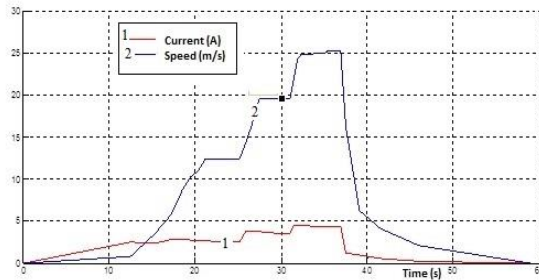
Fig. 16: Running the vehicle in flat road
