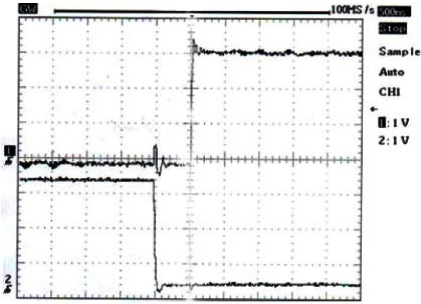
Fig. 11: Dead time between two complementary pulses
