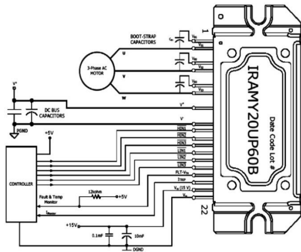
Fig. 8: Typical application connection of IRAMY20UP60B
