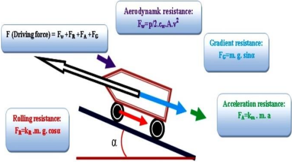
Fig. 1. Representation of all forces acting on EV
