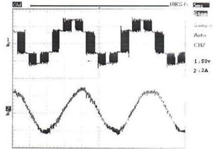
Fig. 15: Wave form of the phase voltage and current for f = 50 Hz with a load torque
