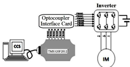
Fig. 5: The block diagram of the open loop control system
