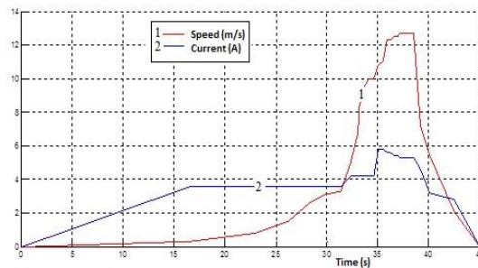
Fig. 17: Running the vehicle in a graded road
