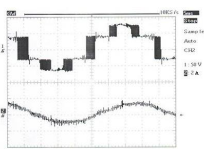
Fig. 14: Wave form of the phase voltage and current for f = 25 Hz with a load torque
