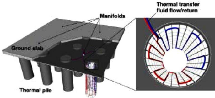
Fig. 11: Principle of a geothermal pile installation [18]
