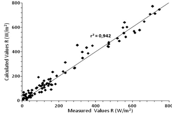
Fig. 5: Comparison between measured and predicted outside global solar radiation R ( \text{W/m}^2 )
