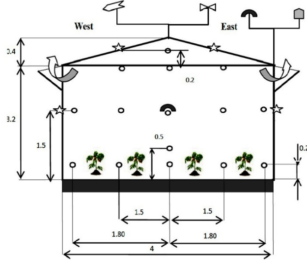
Fig. 1: Sketch of the experimental greenhouse showing the location of the sensors (All the distances are in linear meter)
