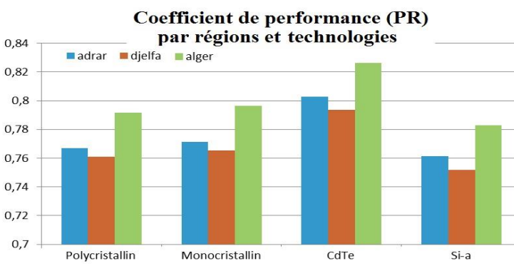
Fig. 5: Coefficient de performance
