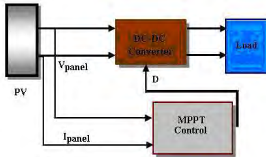
Fig 3: Photovoltaic system
