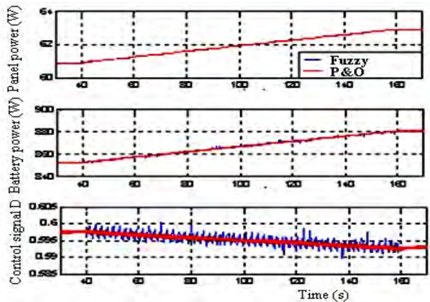
Fig. 16: Fuzzy and P&O controller responses: for a slow (120 s) temperature decrease (30 °C to 20 °C) at 1000 W/m 2 of solar insolation
