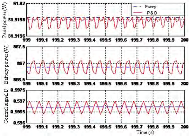
Fig. 10: Wave shape in steady state of the panel and battery power and of the duty ratio signals for a sampling rate of 100 Hz ( T = 25\text{ }^{\circ}\text{C} and S = 1000\text{ W/m}^2 )
