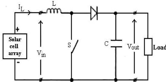
Fig. 6: Basic circuit of the boost chopper
