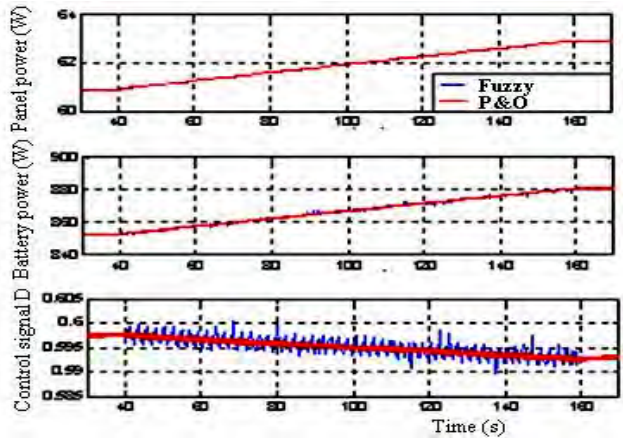
Fig. 15: Fuzzy and P&O controller responses: for a slow (120 s) temperature increase (20 °C to 30 °C) at 1000 W/m 2 of solar insolation
