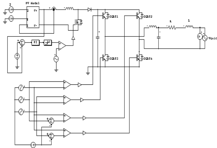
Fig. 5: Block simulation of inverter grid connected
