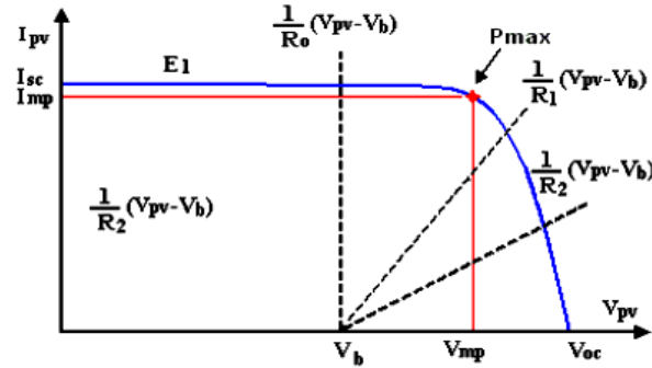
Fig. 6: Source-load characteristics
