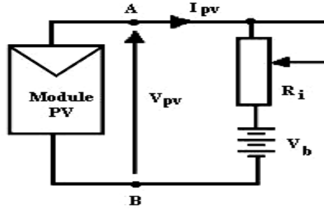
Fig. 5: Direct electric connection between a module and a battery.
