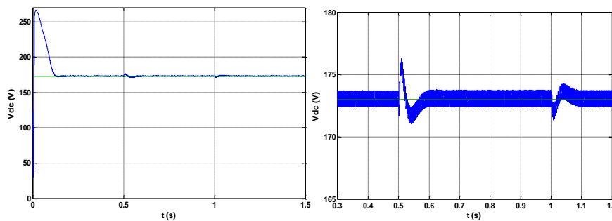
Fig.6. DC bus voltage and its reference.
