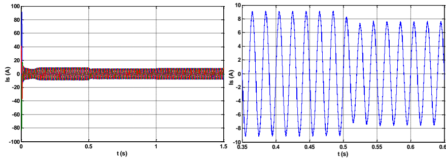
Fig.7. Source current.
