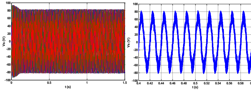
Fig.8. Source voltage.
