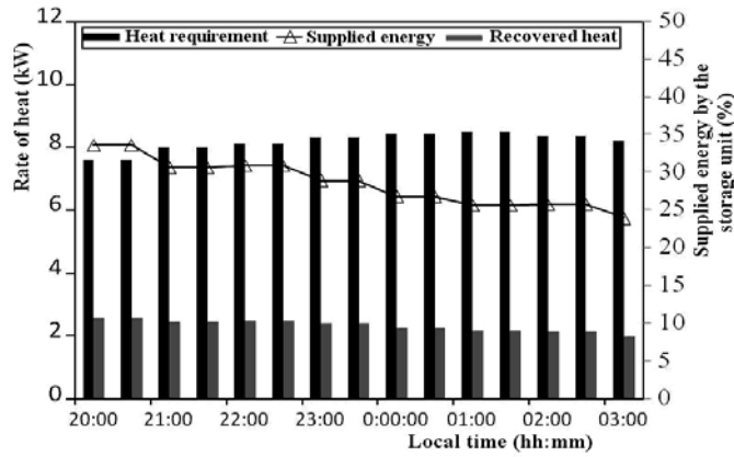
Fig. 10: Changes of the total heat requirement of the tunnel greenhouse and the rate of heat recovered from the heat storage unit during the discharging period
