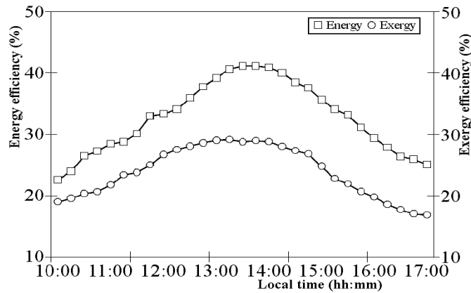
Fig. 7: Change of the net energy and exergy efficiencies for the charging period
