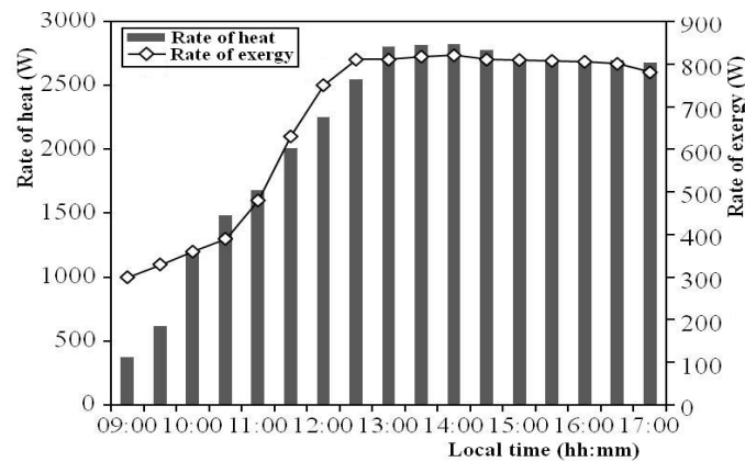
Fig. 6: Rates of heat and thermal exergy stored in the heat storage unit during the charging period
