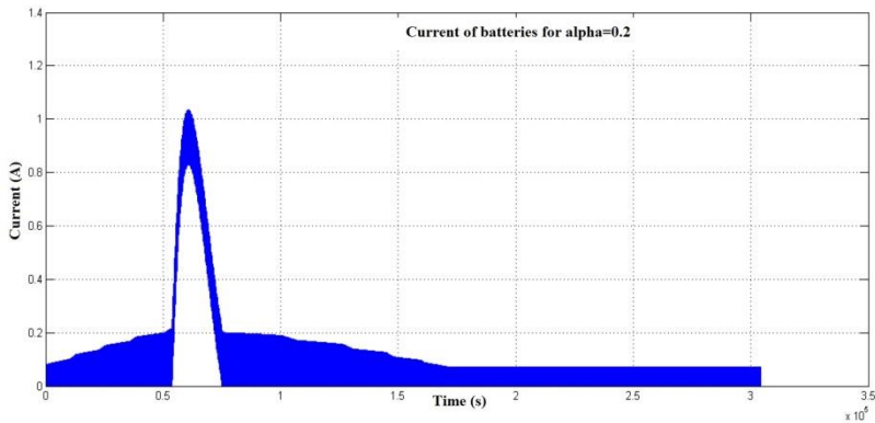
Fig. 5: Simulations show the courant of the batterie for duty cycle alpha = 0.2
