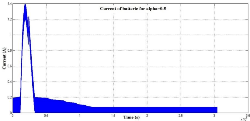
Fig. 4: Simulations show the courant of the batterie for duty cycle alpha = 0.5
