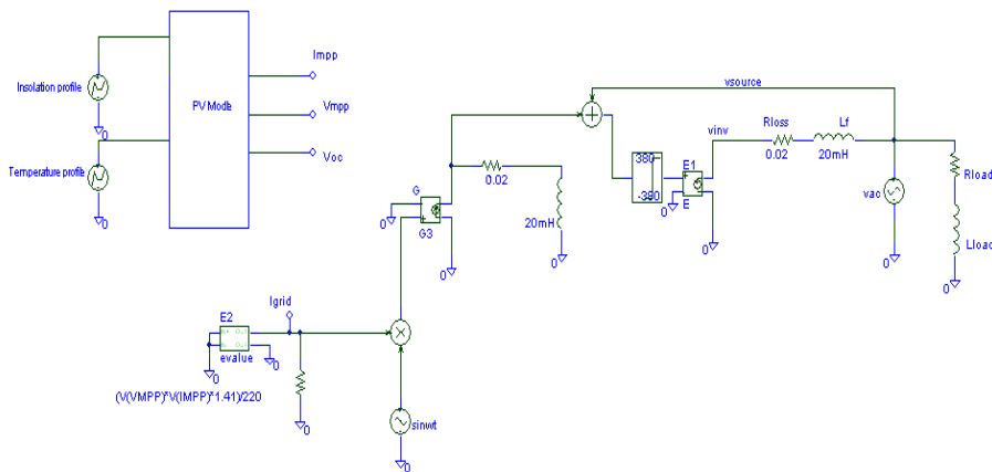
Fig. 12: Pspice schematic of PV grid connected inverter
